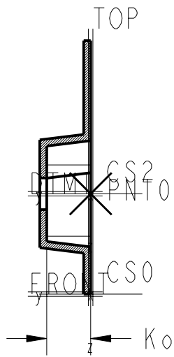
SECTION B-B
